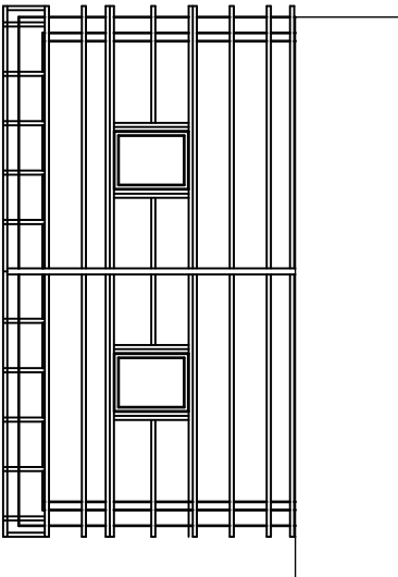
PROPOSED ROOF STRUCTURE PLAN 1:100
