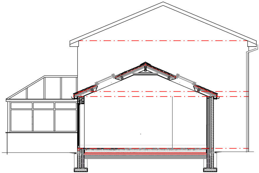
PROPOSED SECTION 1:100
