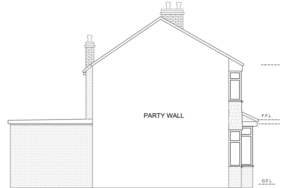
EXISTING SIDE ELEVATION (NORTH EAST)
