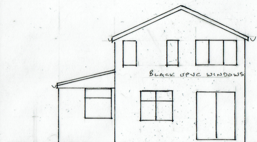
REAR ELEVATION
