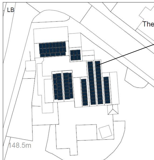
Figure 2: Proposed solar PV layout
