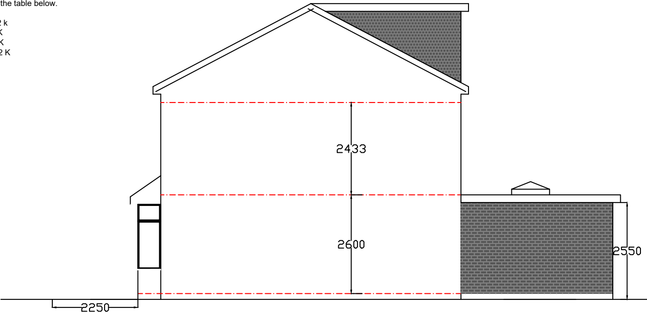
Elevation From No 10
