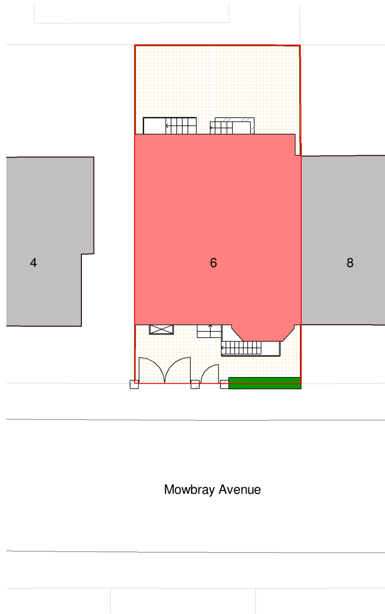
2 Site - Proposed 1 : 200
