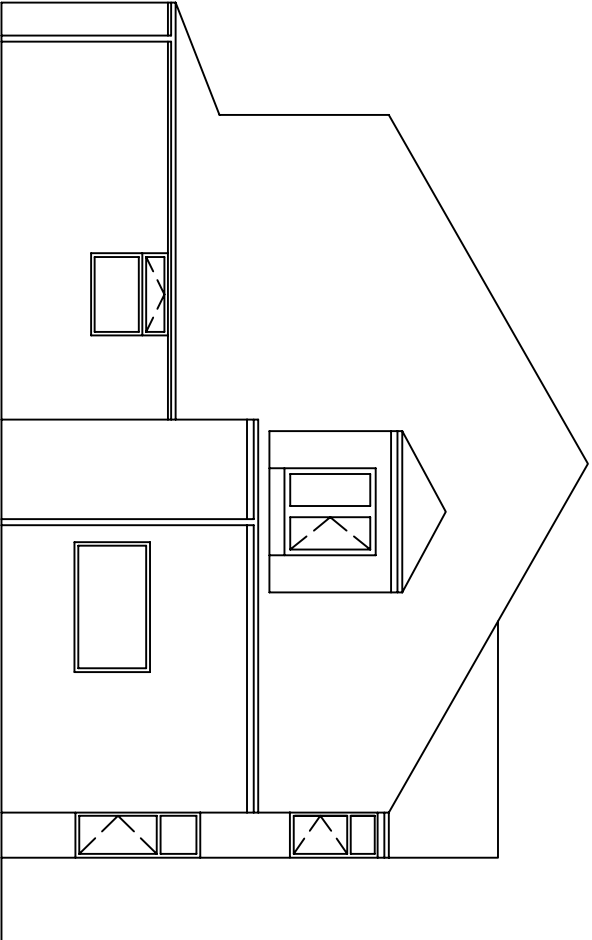
Side Elevation
