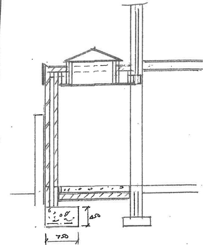
BOUNDARY WALL TYPICAL FOUNDATION
