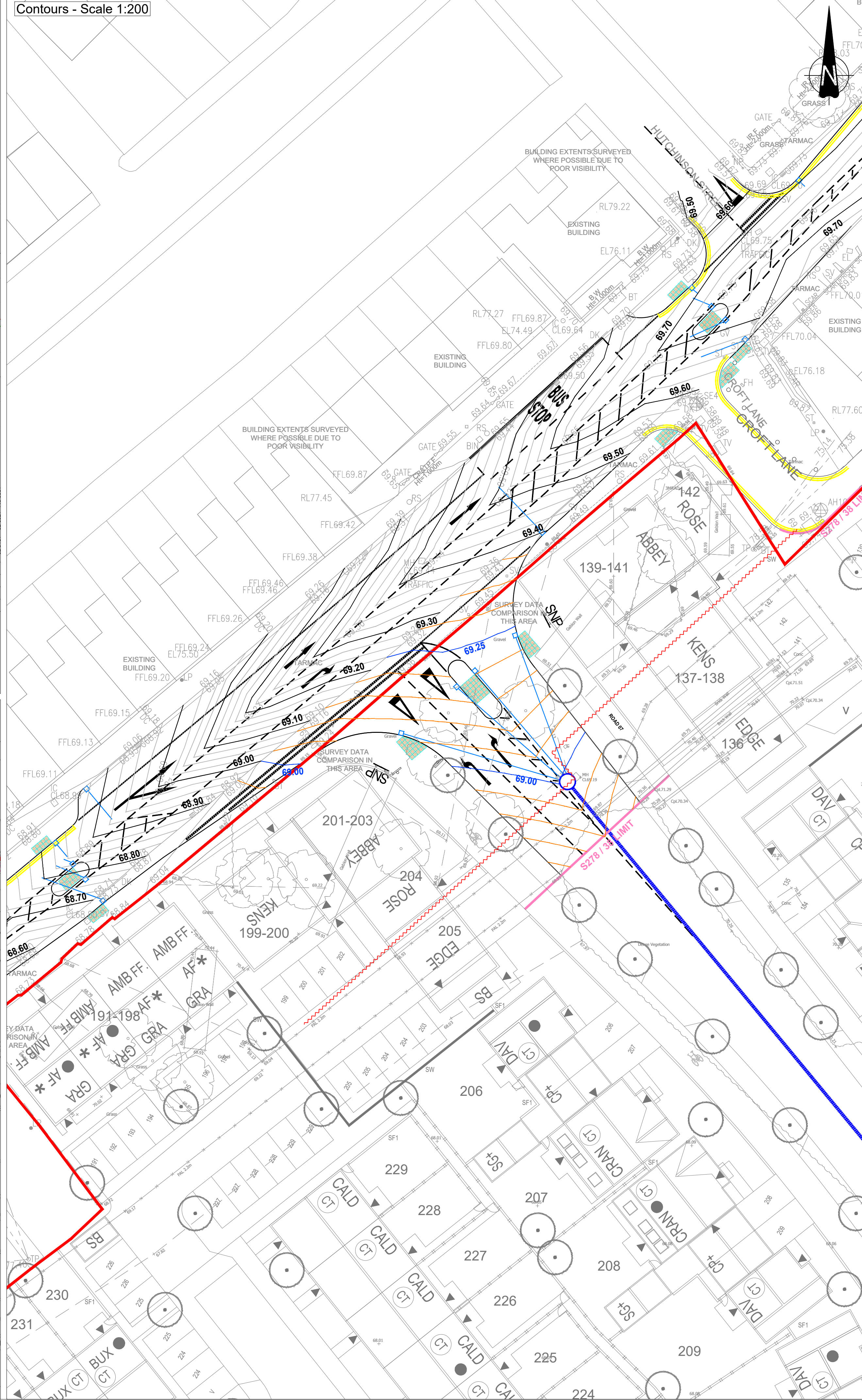
Contours - Scale 1:200
