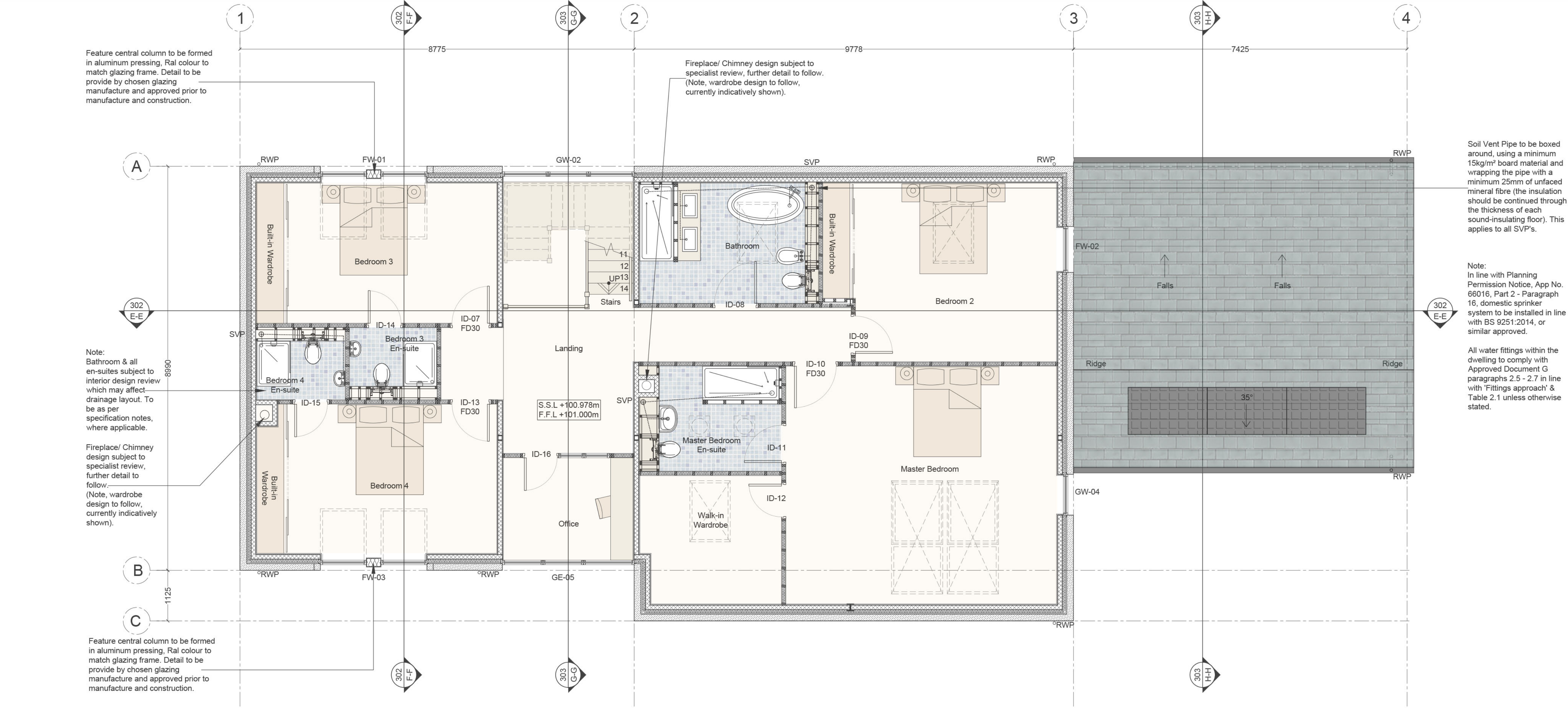
Detached House Proposed First Floor GA Plan Scale 1:50
