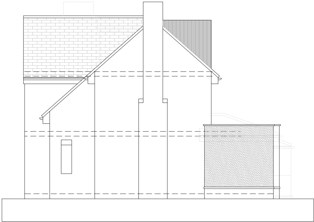
PROPOSED GABLE ELEVATION (1:100)
