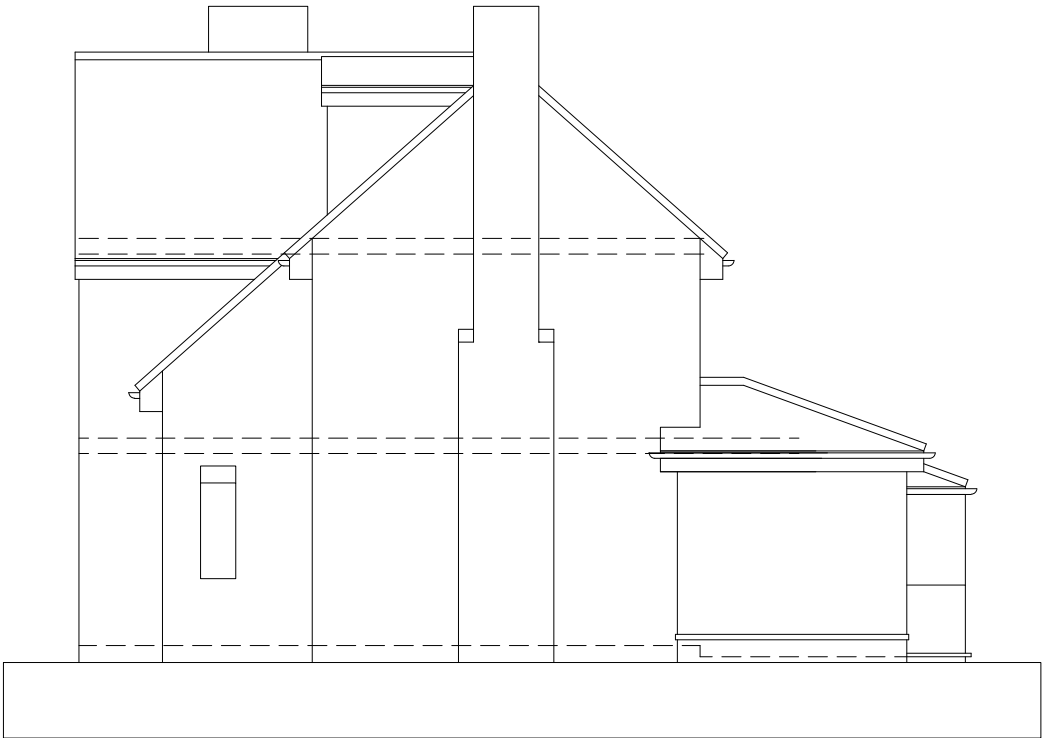
EXISTING GABLE ELEVATION (1:100)
