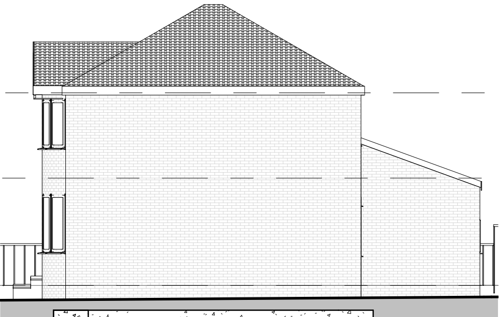
Existing Elevation North 1 : 100
