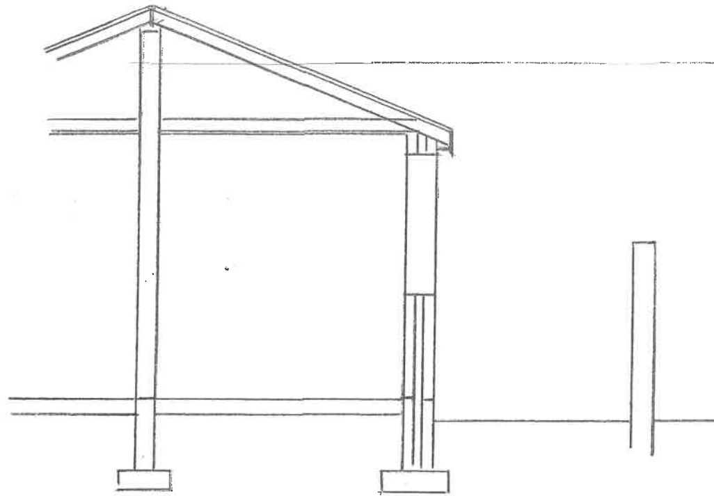
EXISTING SECTION THRU KITCHEN
