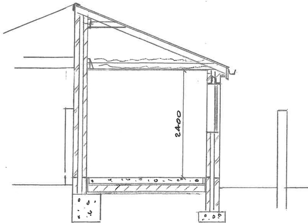
PROPOSED SECTION THRU EXTENSION
