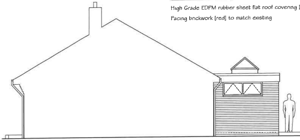
PROPOSED SOUTH EAST SECTIONAL ELEVATION 1:100 @ A4 [A5 VIEWED FROM NO 4]
