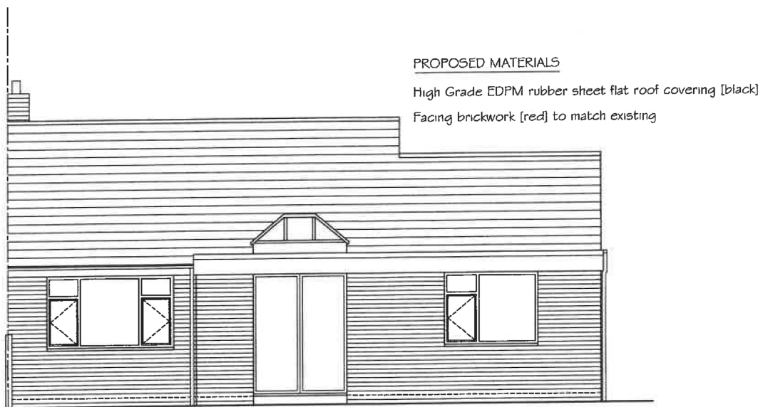
PROPOSED NORTH EAST ELEVATION 1:100 @ A4
