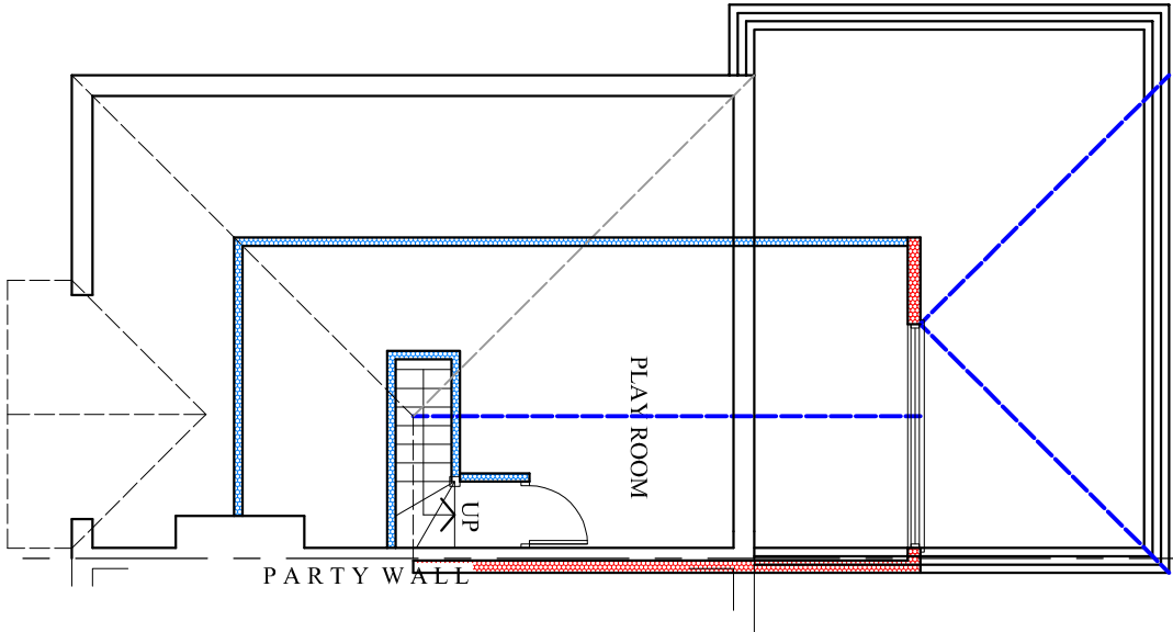
PROPOSED LOFT PLAN
