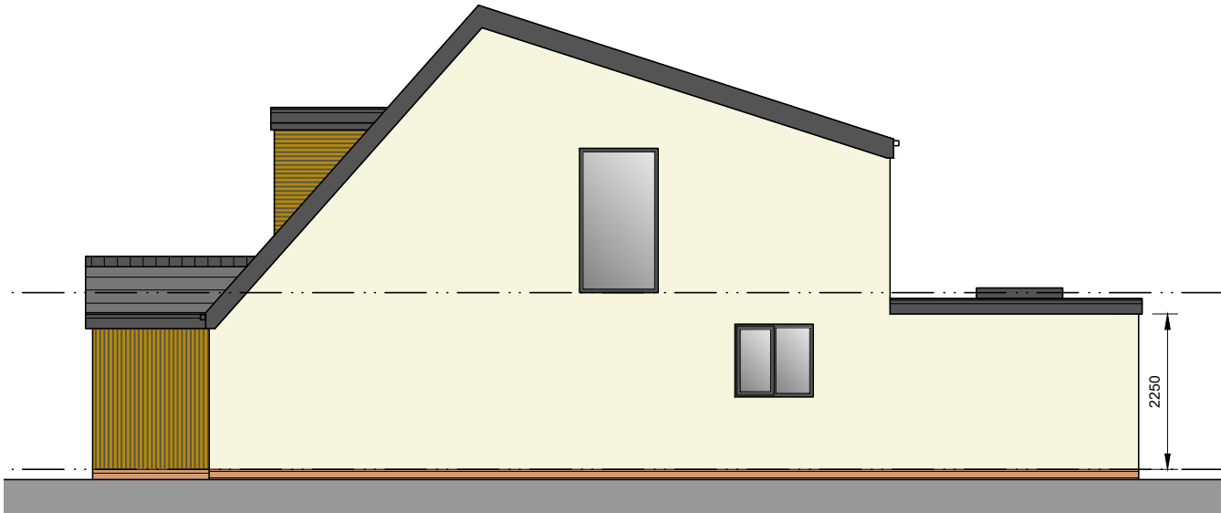
East Facing Side Elevation
