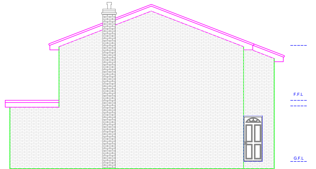
EXISTING SIDE ELEVATION (NORTH WEST)
