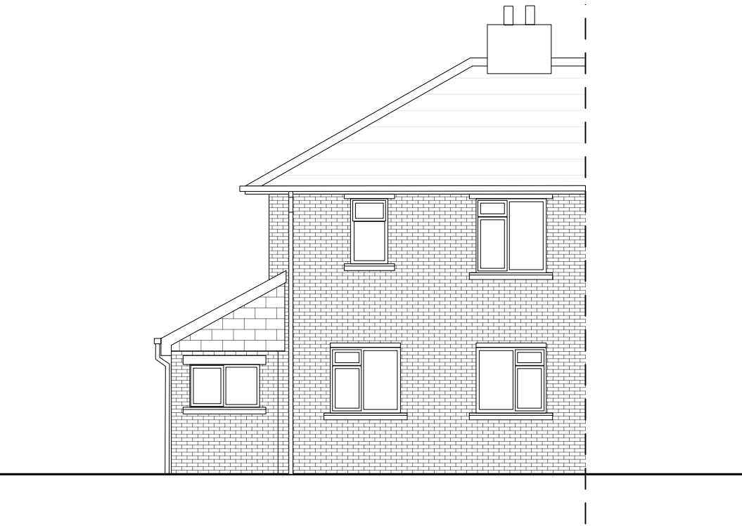
NORTH EAST (REAR) ELEVATION
