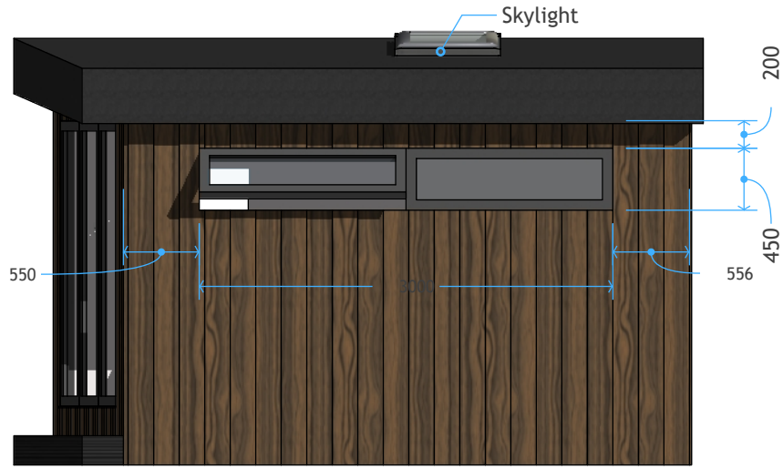
0 Front Elevation A01
