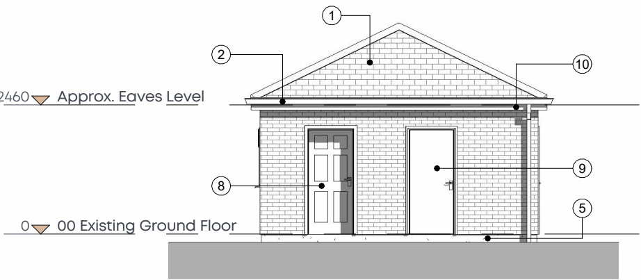
Existing Rear Elevation - Typical Twin
