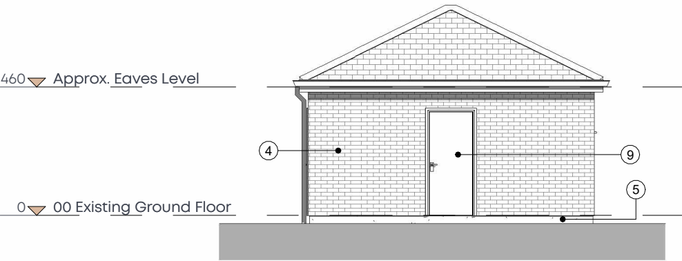
Existing Side Elevation 02 - Typical Twin
