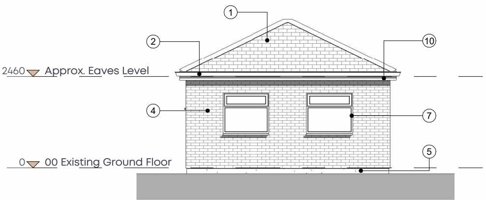
Existing Side Elevation 01 - Typical Twin
