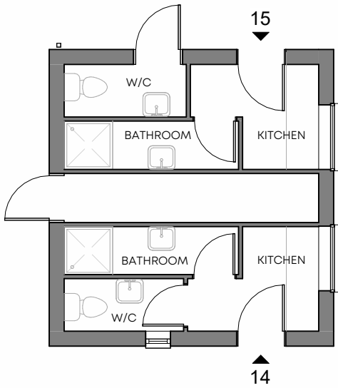
00 Existing Ground Floor -Twin (14 & 15)
