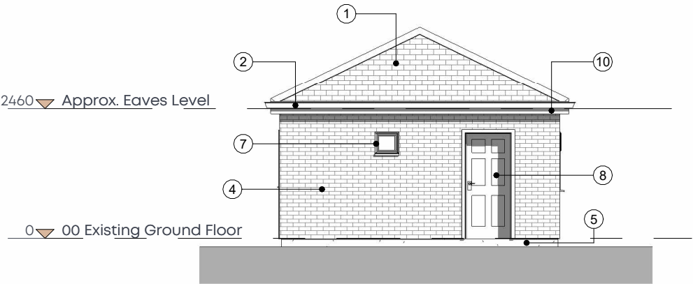
Existing Front Elevation - Typical Twin
