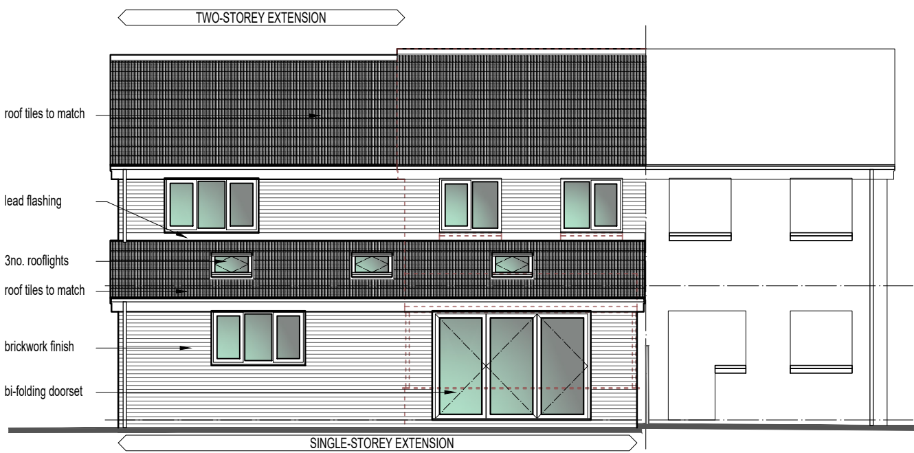
REAR ELEVATION
