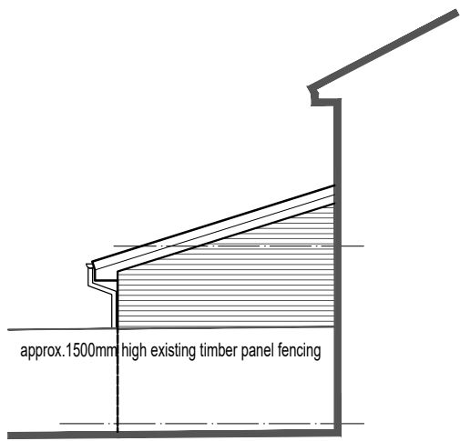
SIDE ELEVATION (view from 59 Lakeland Crescent)
