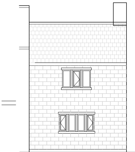
EXISTING FRONT ELEVATION 1:100 @ A3
