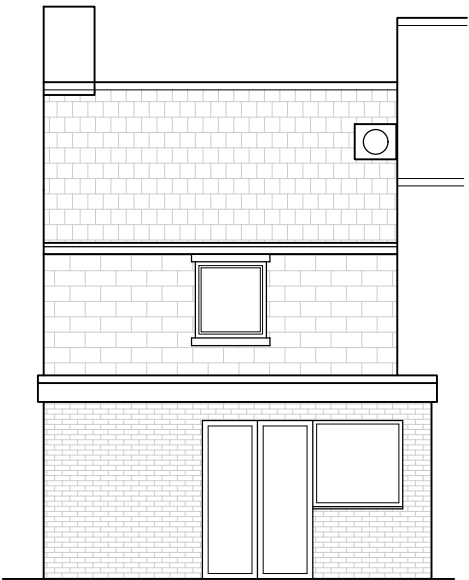
EXISTING REAR ELEVATION 1:100 @ A3
