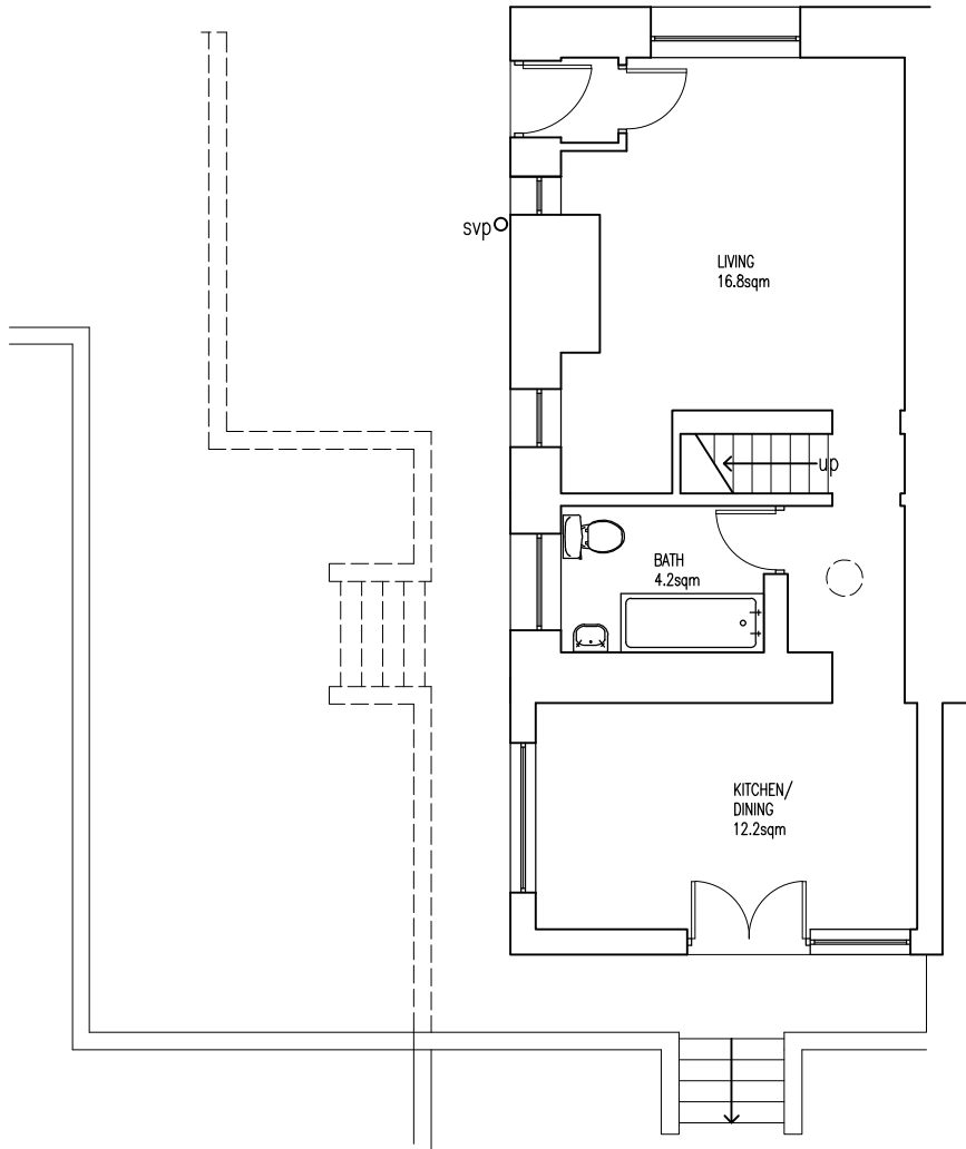
EXISTING GROUND FLOOR PLAN 1:100 @ A3
