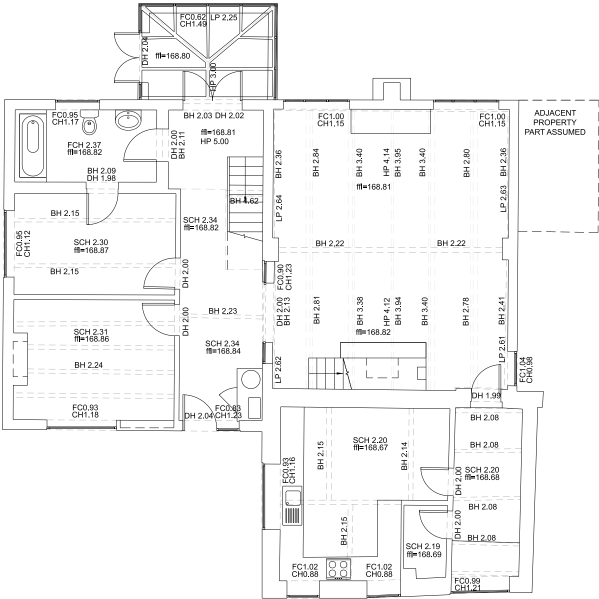
GROUND FLOOR
