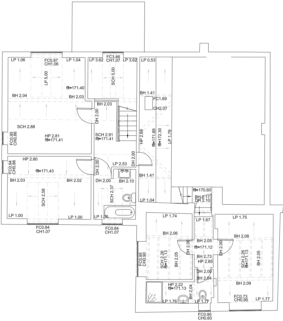
FIRST FLOOR
