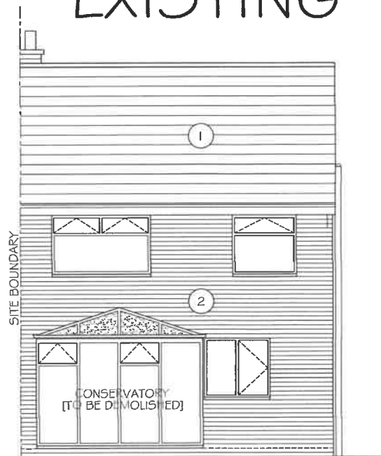
EXISTING NORTH WEST ELEVATION 1:100
