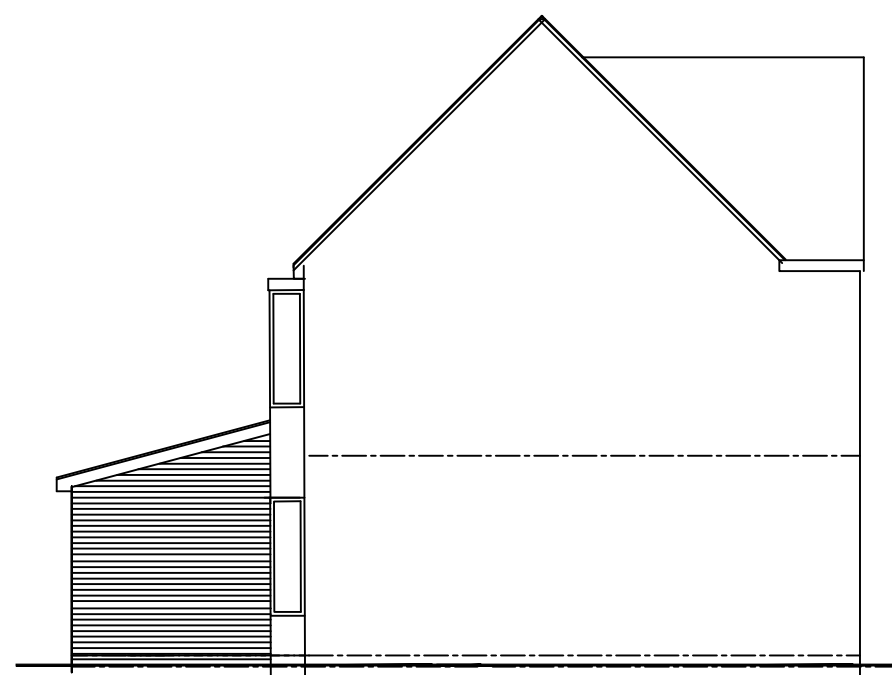
PROPOSED SOUTH (Side) ELEVATION
