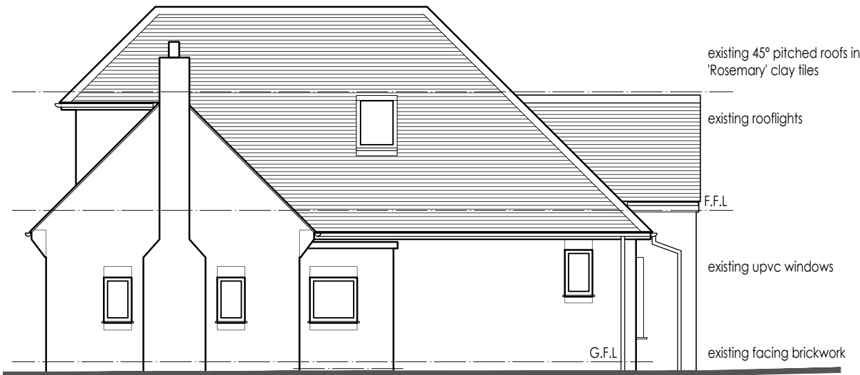
SIDE ELEVATION (facing 9 Crag Avenue)
