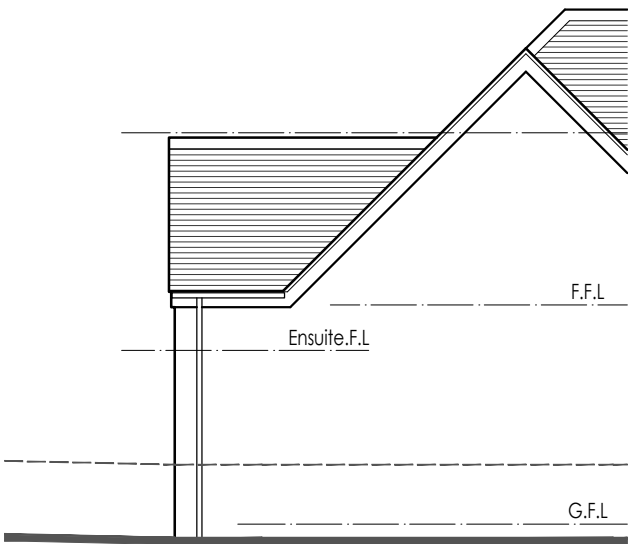
SIDE ELEVATION (facing 13 Crag Avenue)
