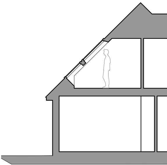
TYPICAL SECTION
