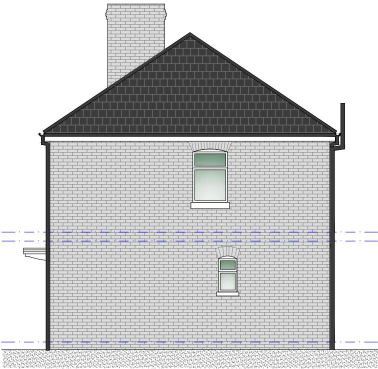
Existing R/H Side Elevation Scale 1:100
