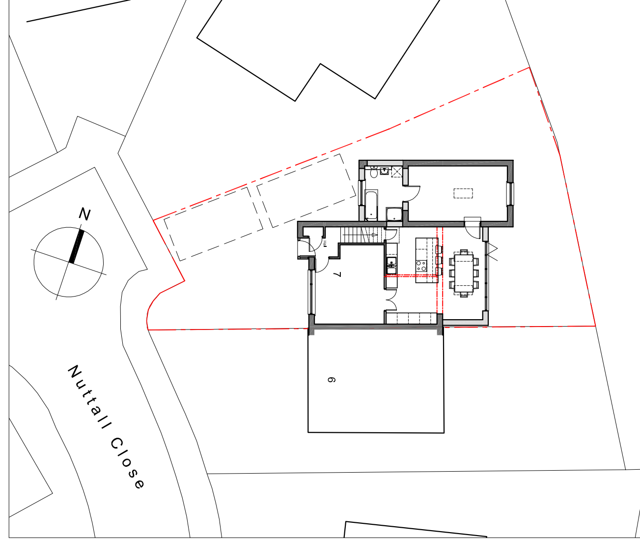
Proposed Site Plan - 1:1200
