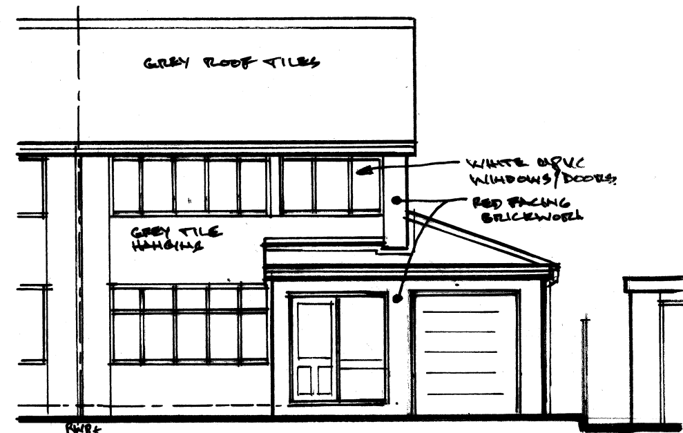
FRONT ELEVATION 1:100
