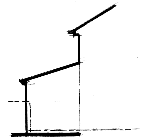
REAR SIDE ELEVATION (TO HAVE NO CHANGE.)
