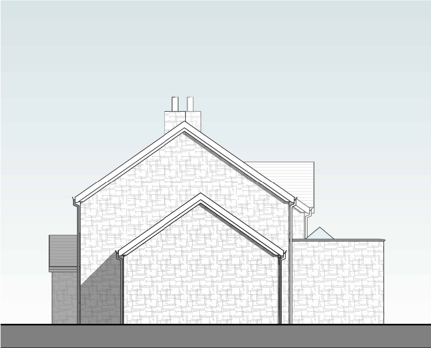
East Elevation 1 : 100
