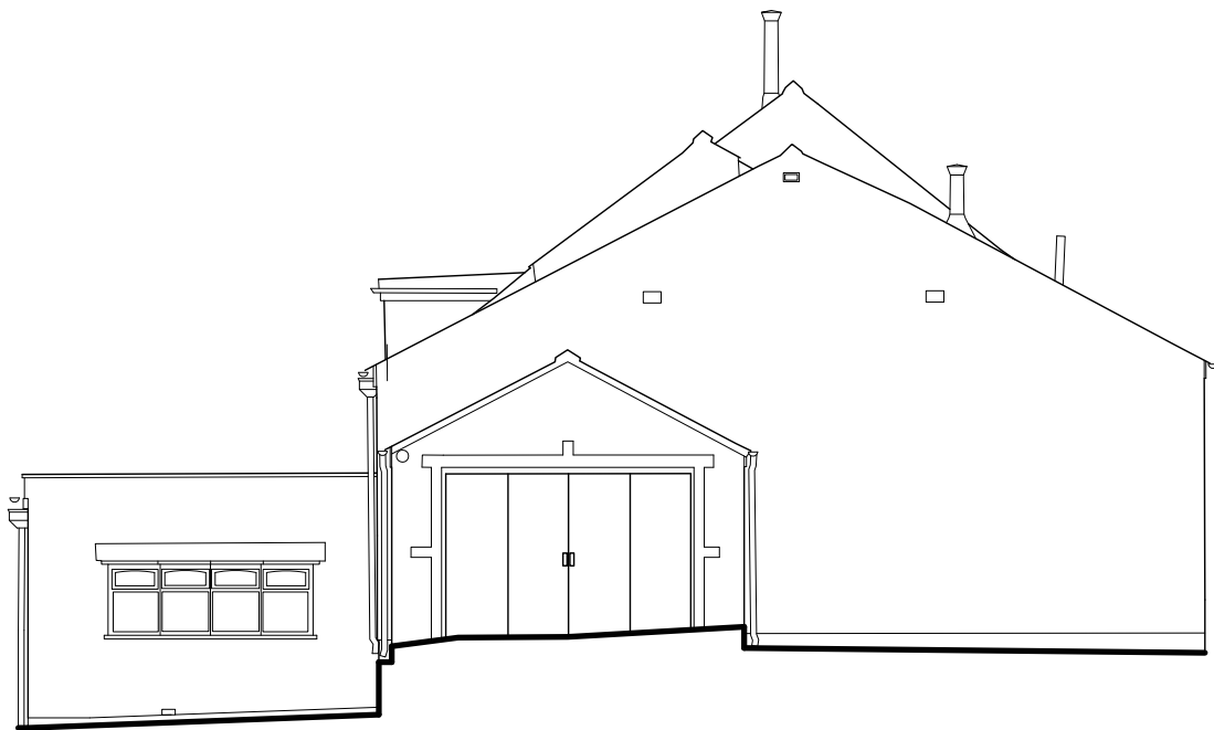
WEST ELEVATION
