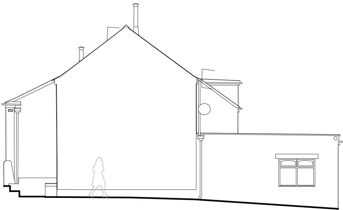
EAST ELEVATION
