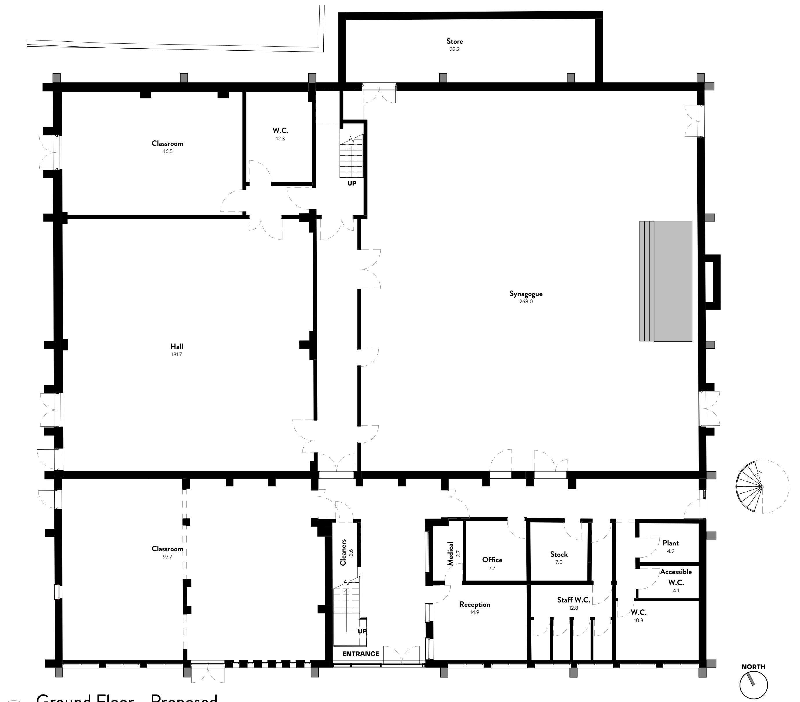
2 Ground Floor - Proposed 1:100
