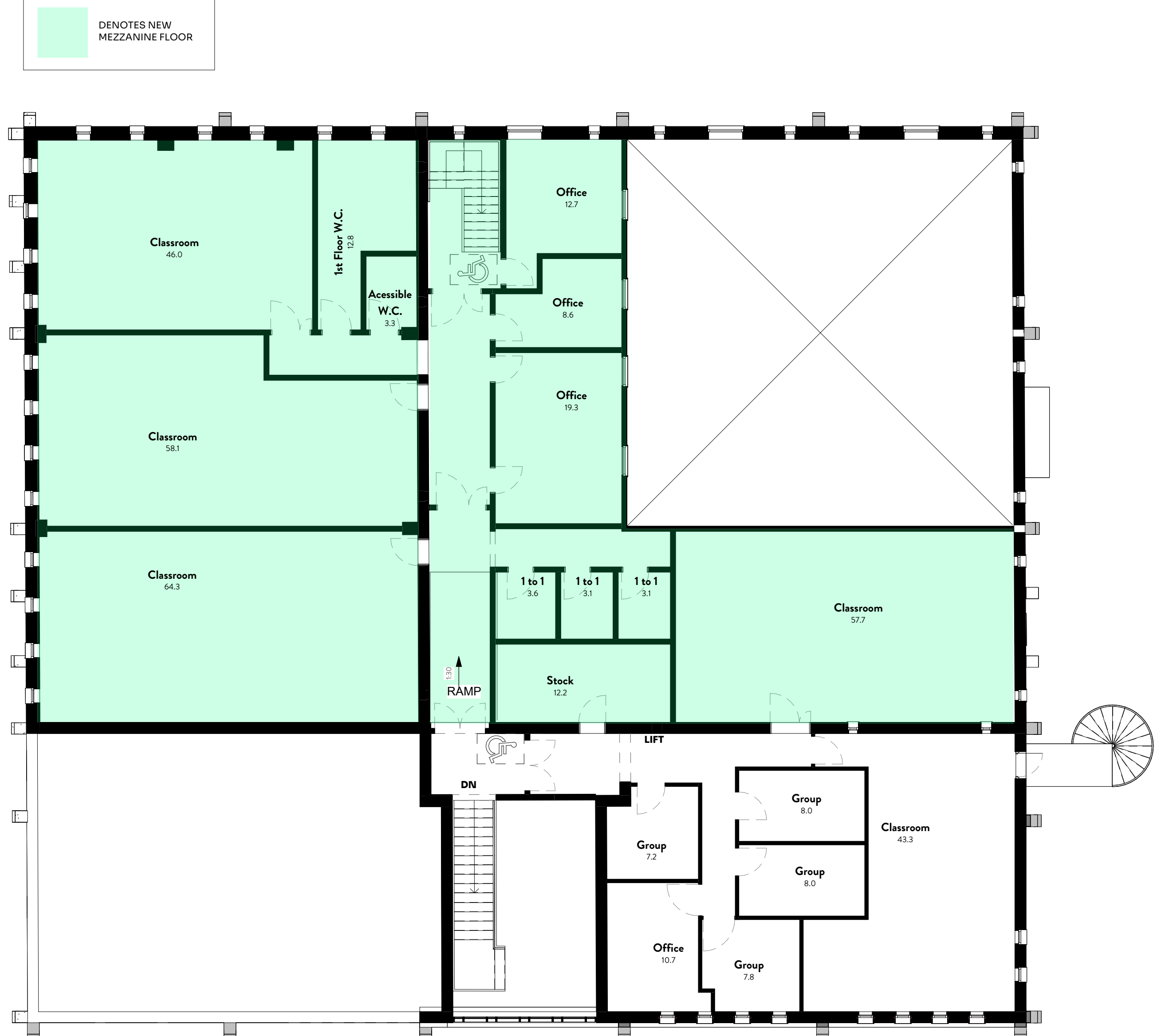
3 First Floor 1:100
