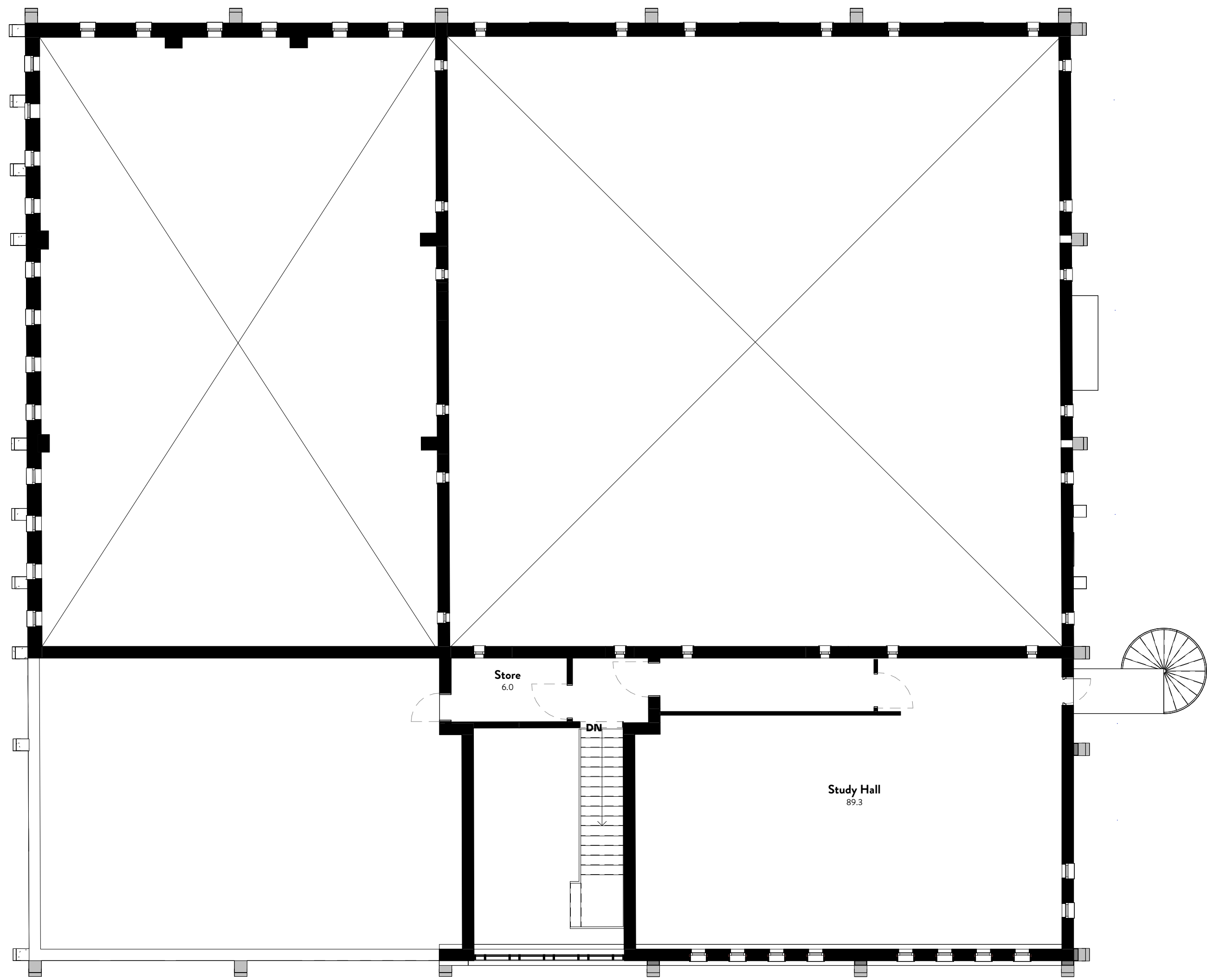
3 First Floor 1:100
