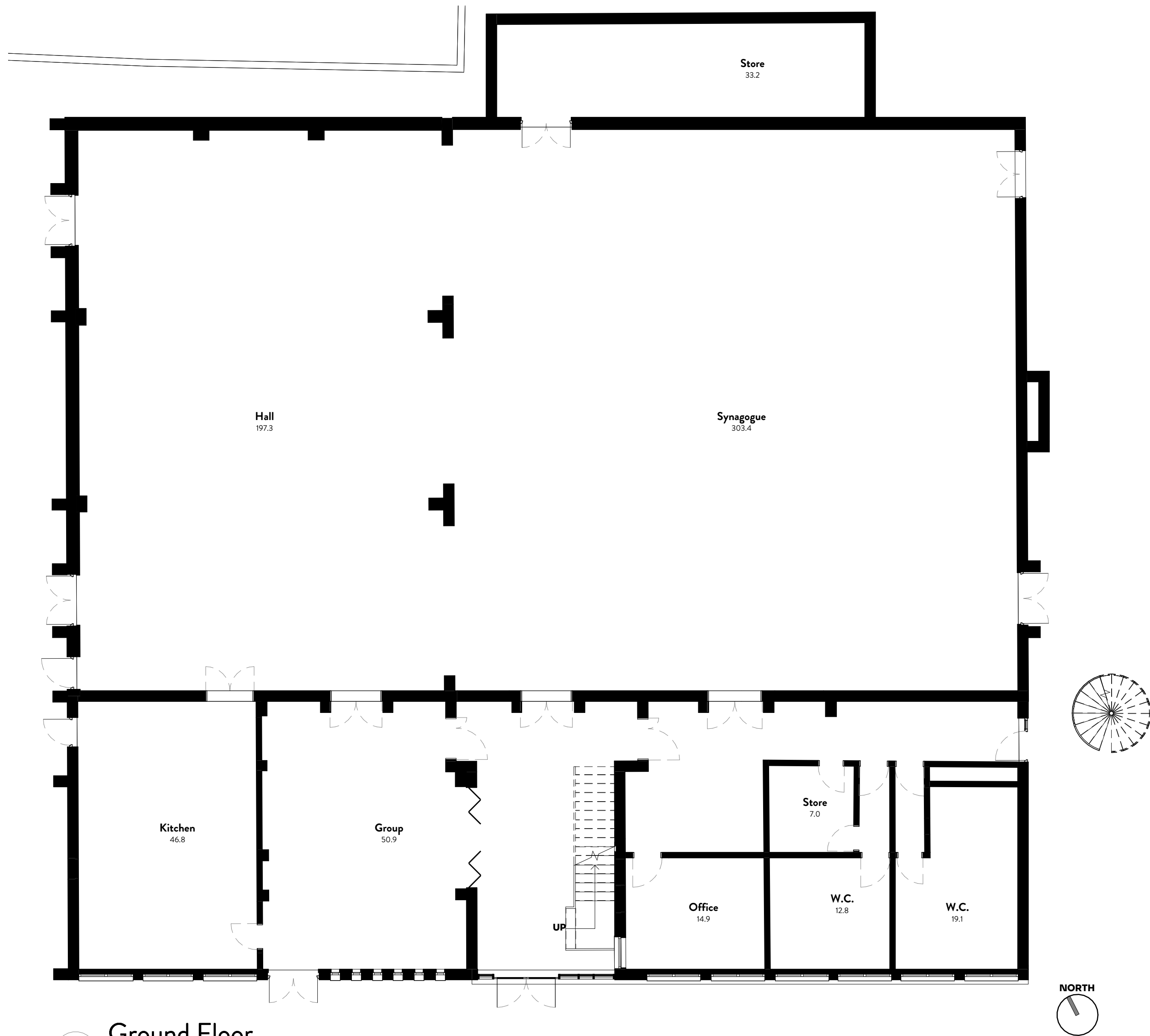
2 Ground Floor 1:100
