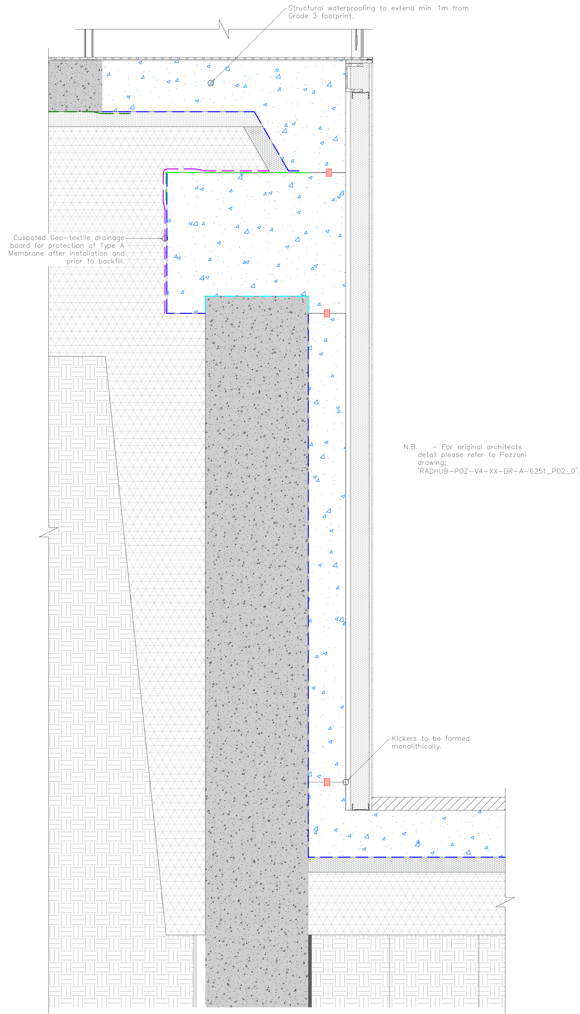
2 Piled Retaining Wall to Intermediate Slab Detail Scale: 1:50
