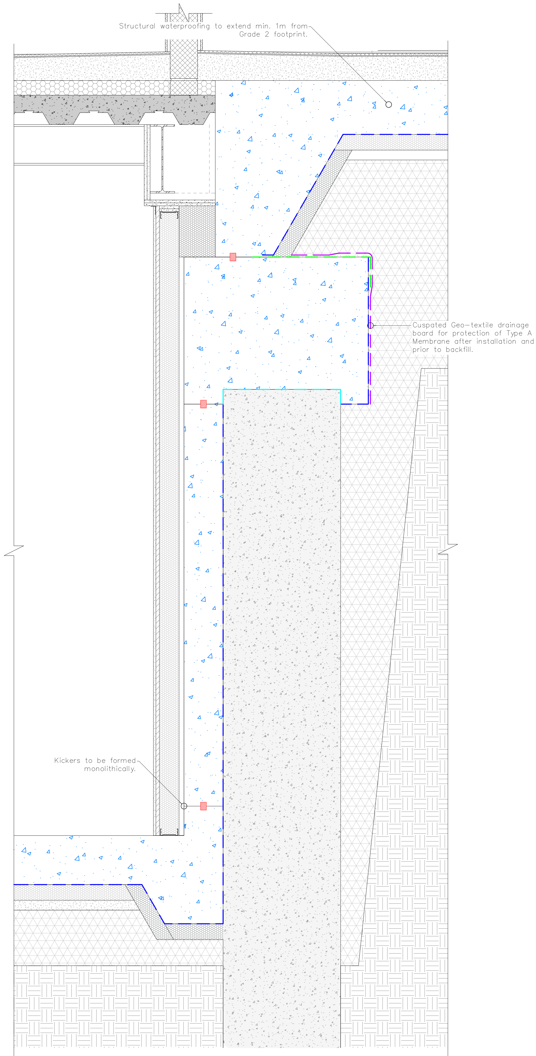
2 Plant Room Piled Retaining Wall to Intermediate Slab Detail Scale: 1:50
