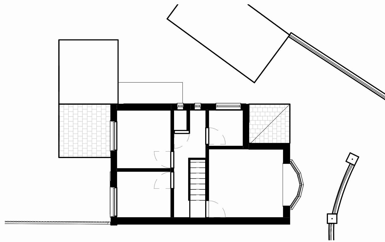
2 Existing First Floor Plan 1 : 100
