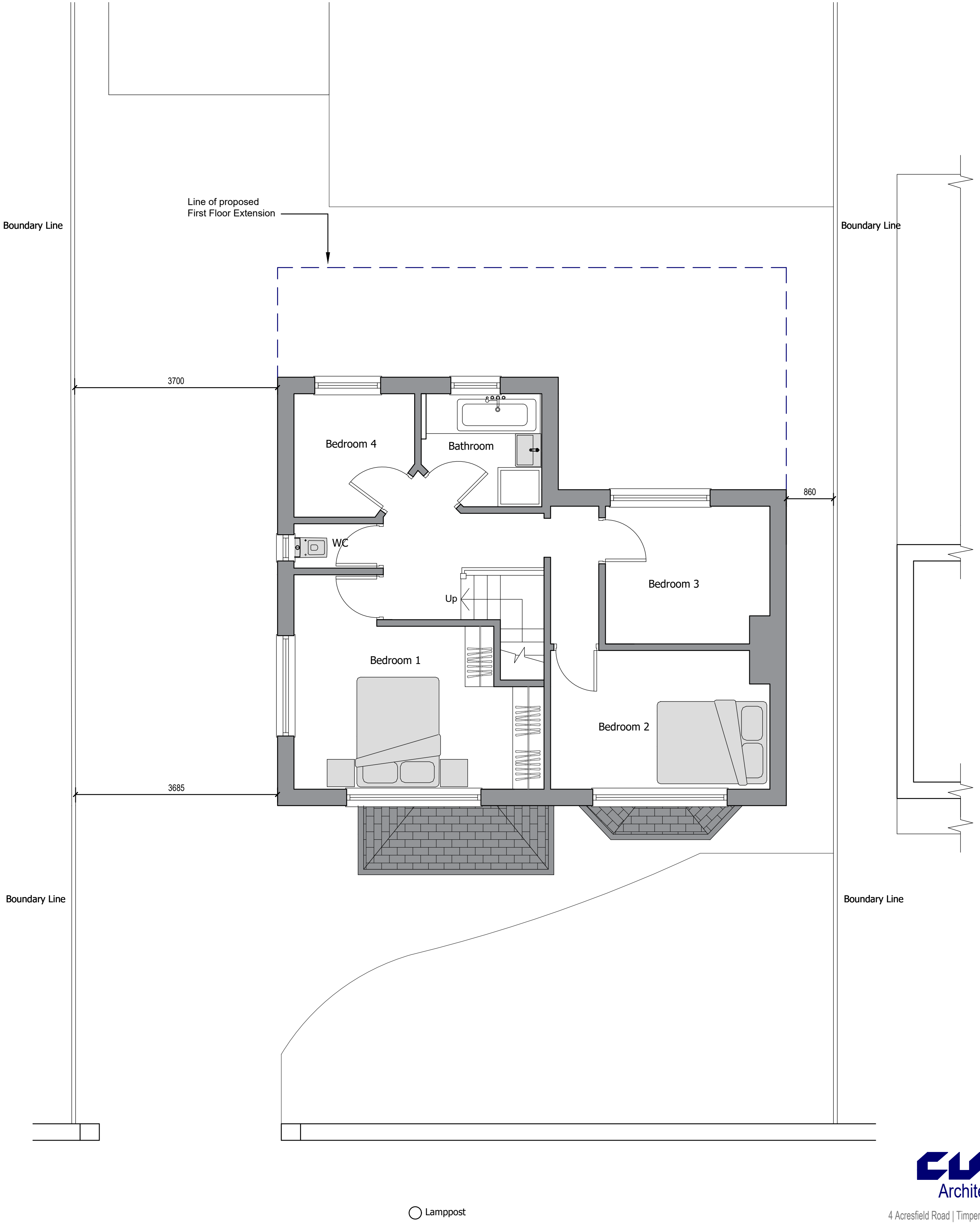
First Floor
