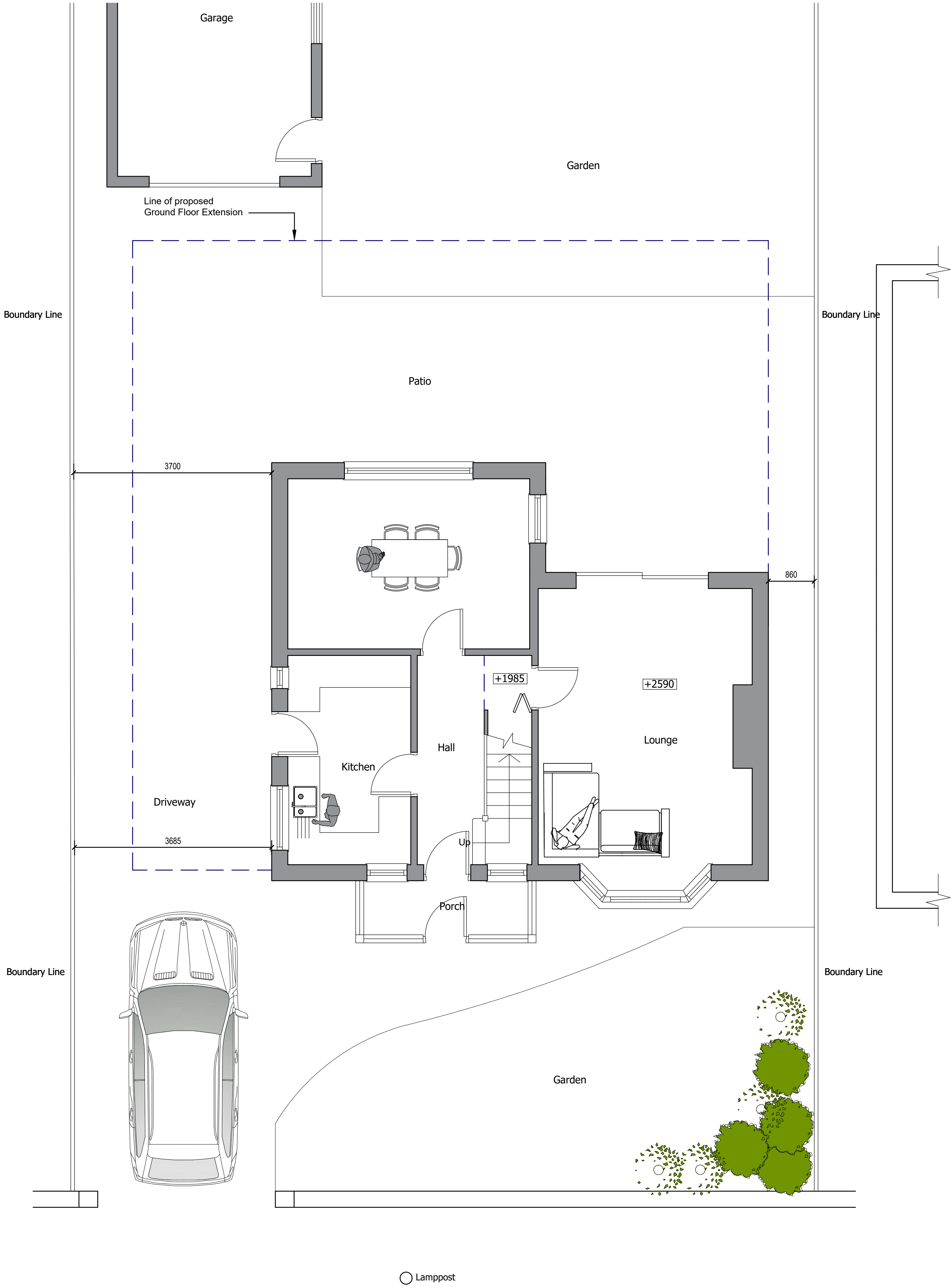
Ground Floor
