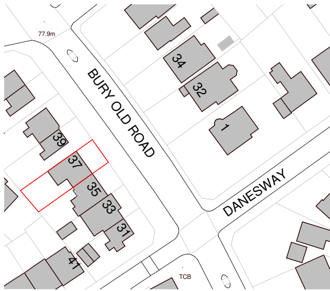
2 Site - Location Plan 1 : 1250 10 0 10 20 30 40 50 SCALE 1250 1: m
