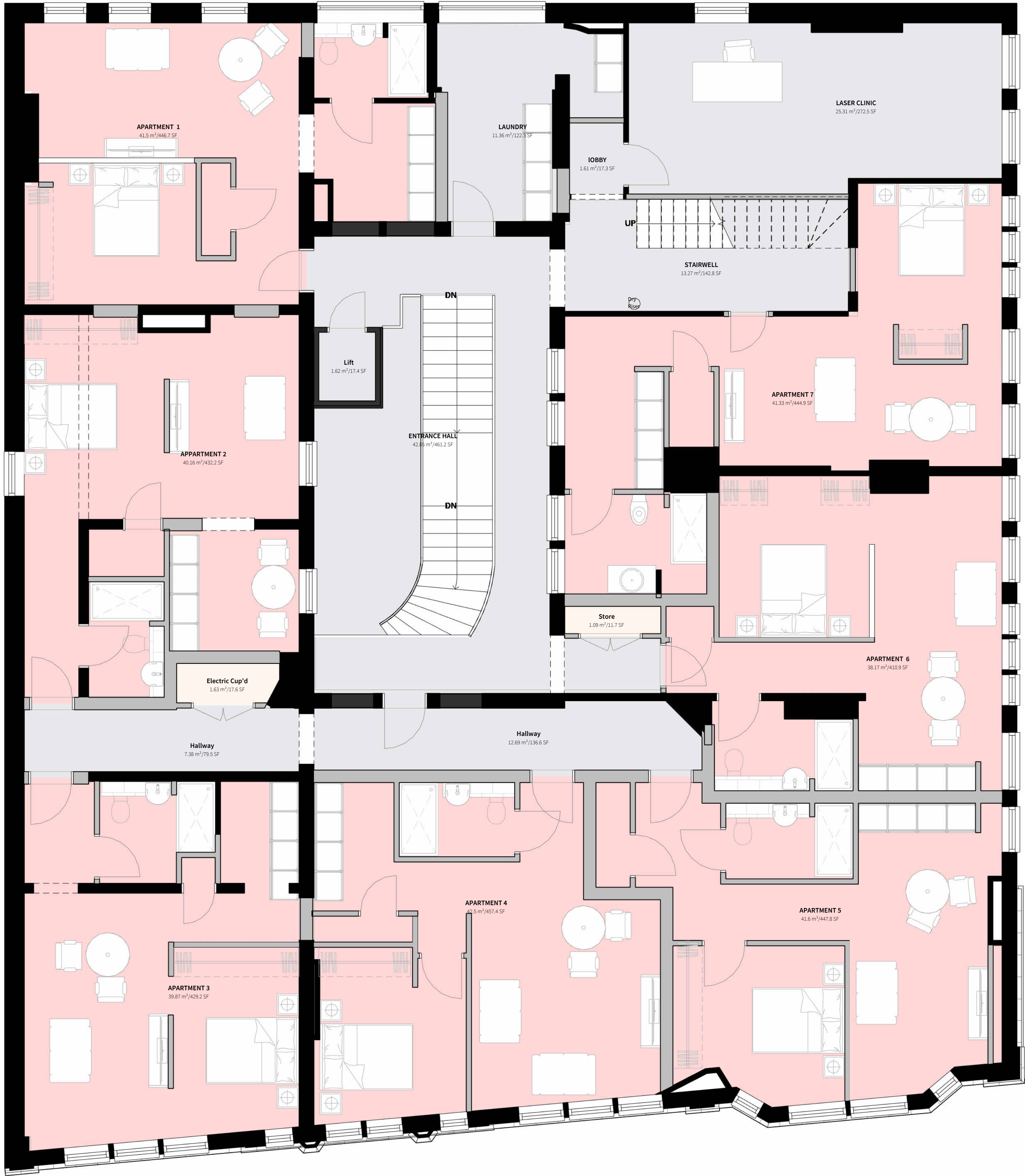
2 Proposed-Plan_01-First 1:50
