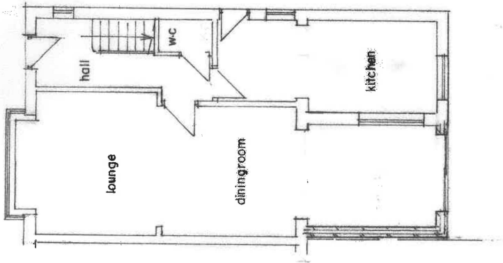
GROUND FLOOR PLAN (PROPOSED)
