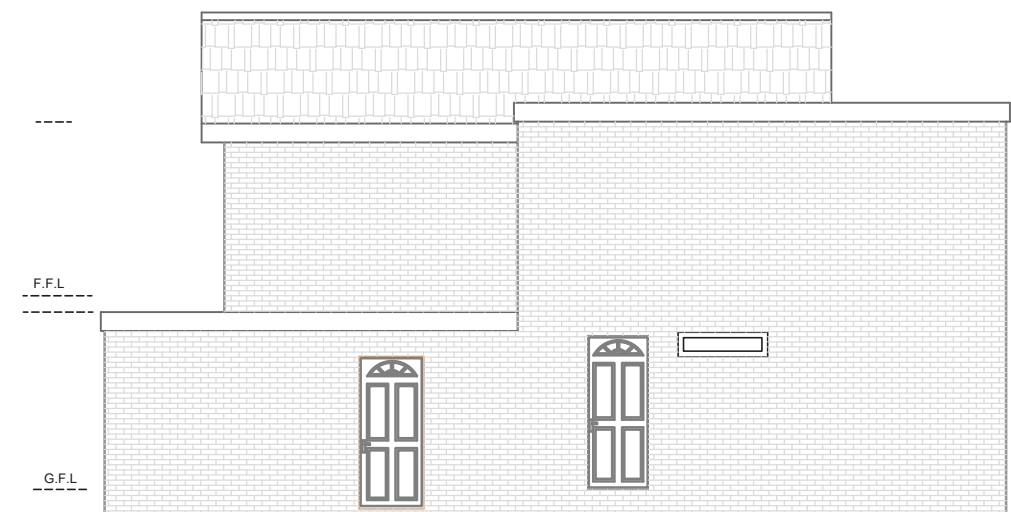
EXISTING SIDE ELEVATION (EAST)
