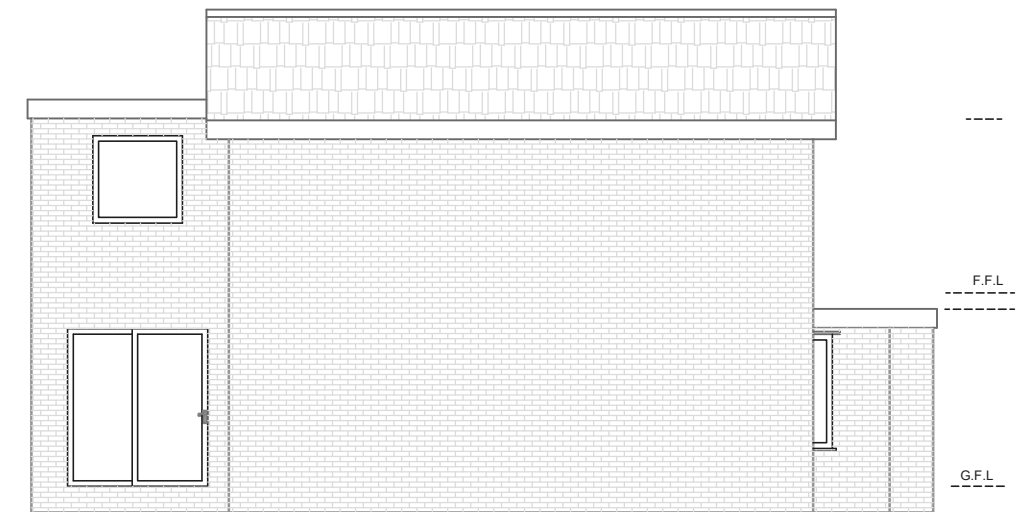
EXISTING SIDE ELEVATION (WEST)
