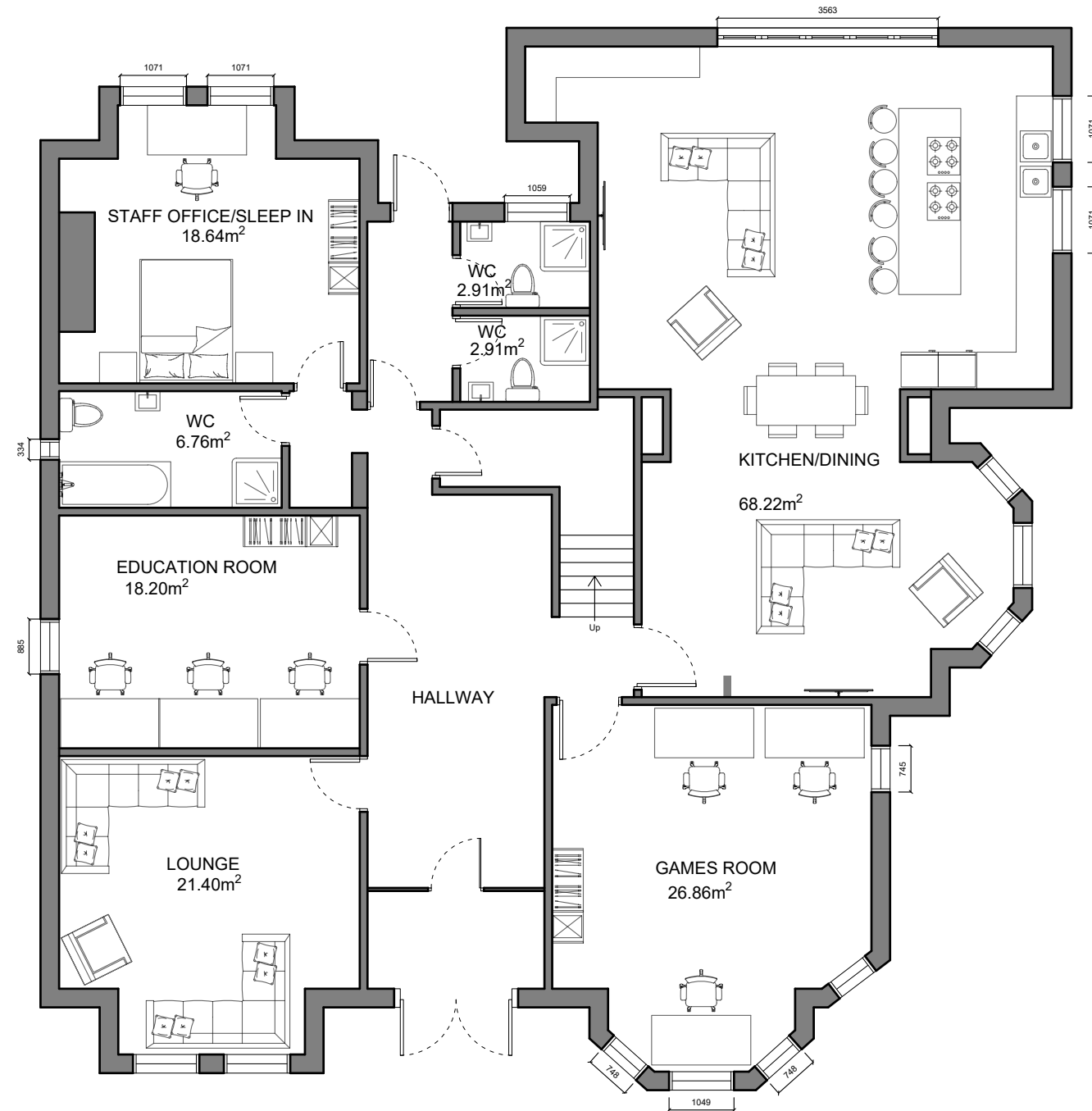
Proposed Ground Floor Plan Revision 1
