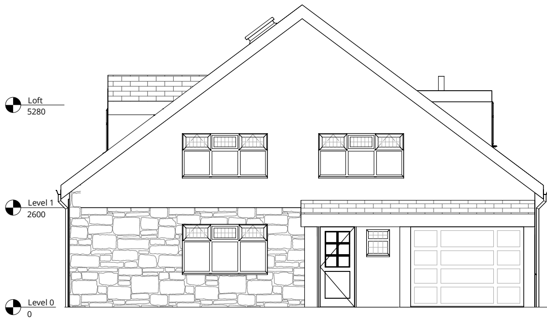
3 Front Elevation 1 : 100
