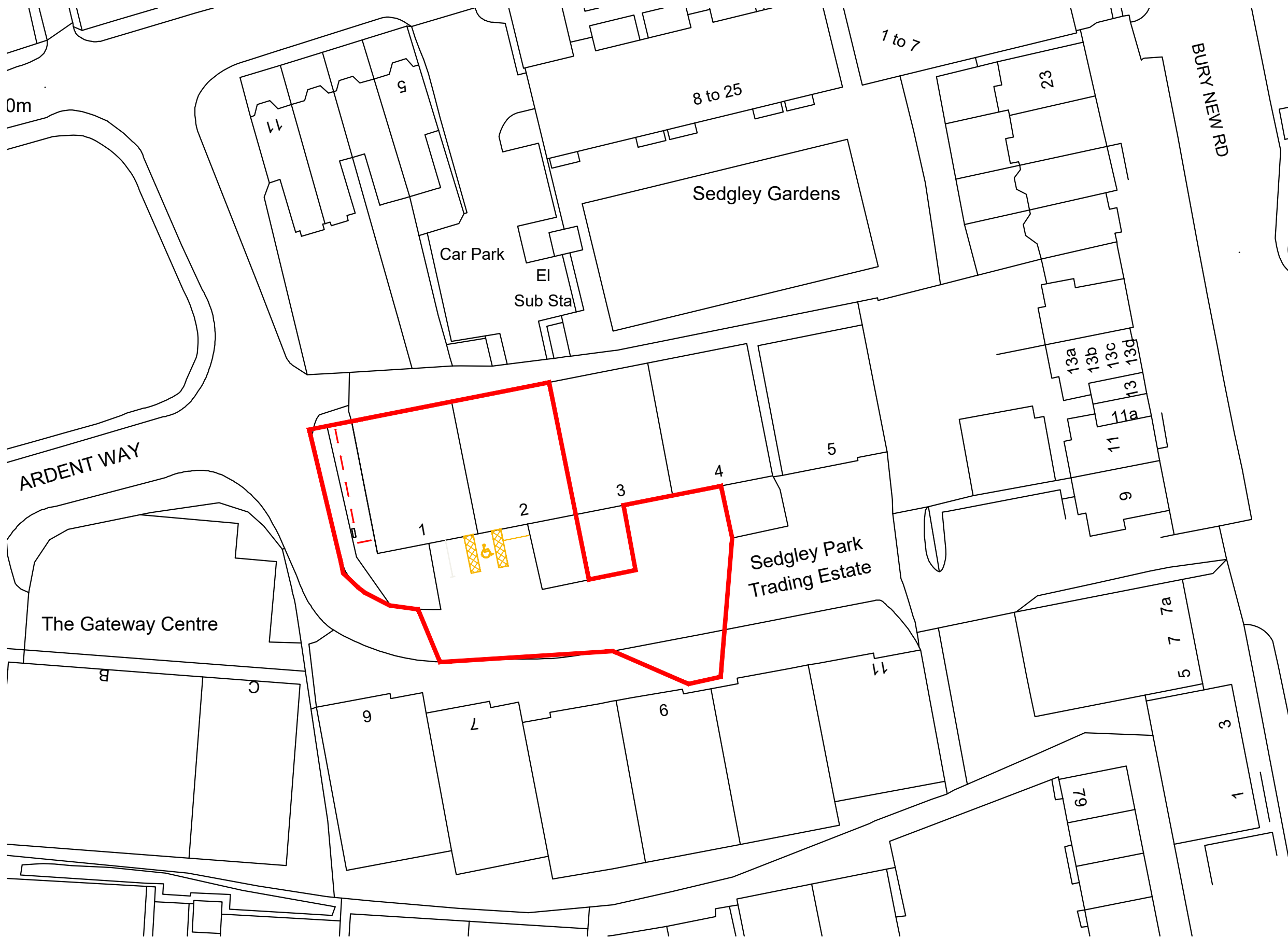
BLOCK PLAN SCALE 1:500 (Site Area shown in red outline) Area within red line boundary = 1263m 2
