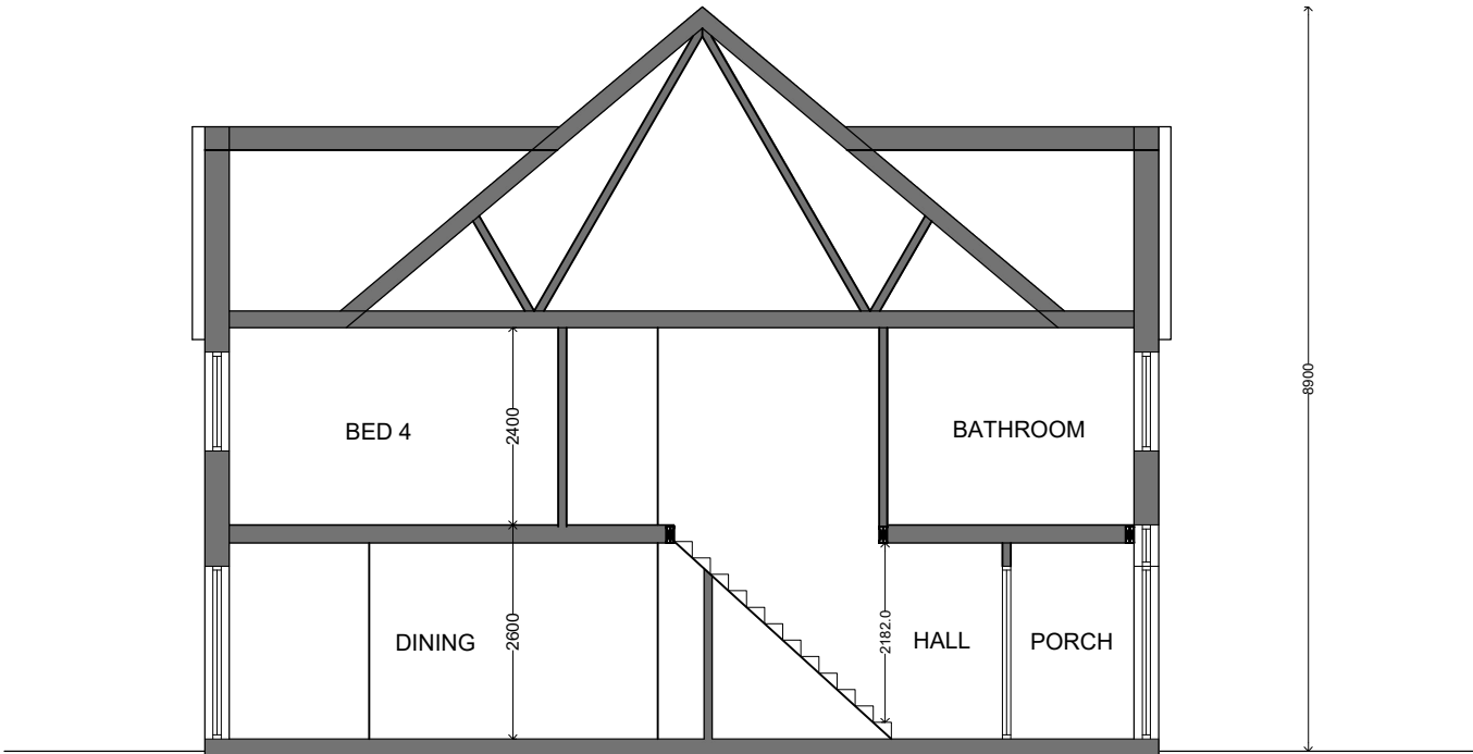
SECTION B-B
