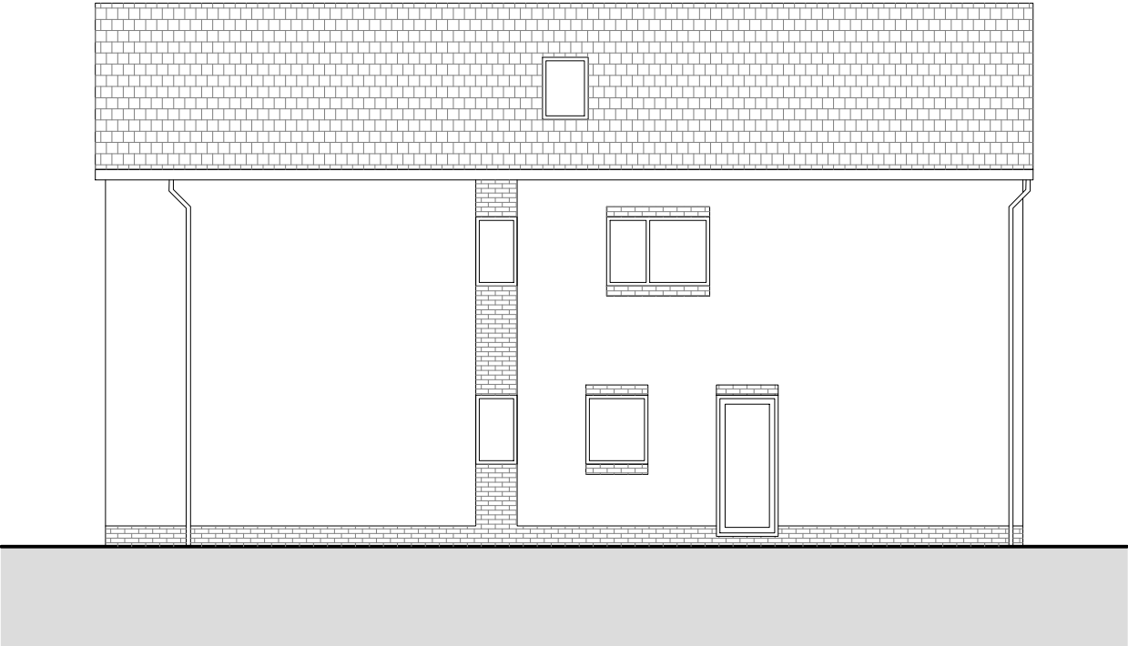
APPROVED SIDE ELEVATION
