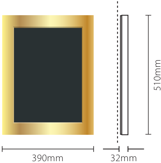
Scale : 1:10 @ A3 Item E. 1no. Brass internally illuminated menu case. G/CI - 1350mm D - 32mm
