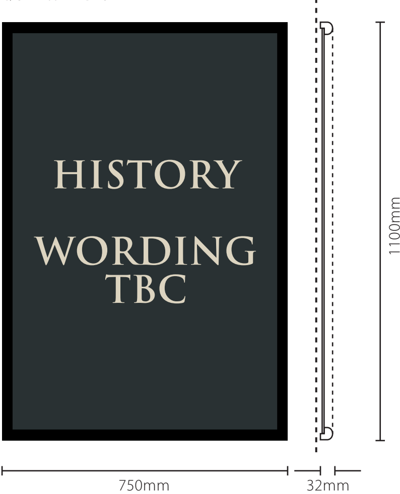
Scale : 1:10 @ A3 Item D. 1no. Sprayed Aluminium amenity board with applied vinyl. G/CI - 1200mm D - 32mm
